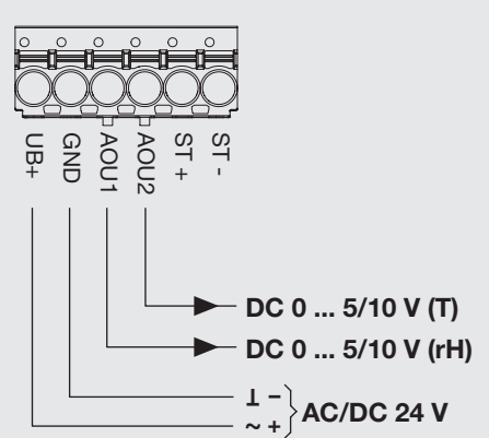
2 x 0...5/10 V
