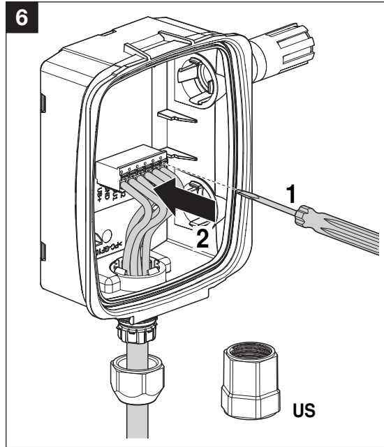
0...5/10 V + ST
