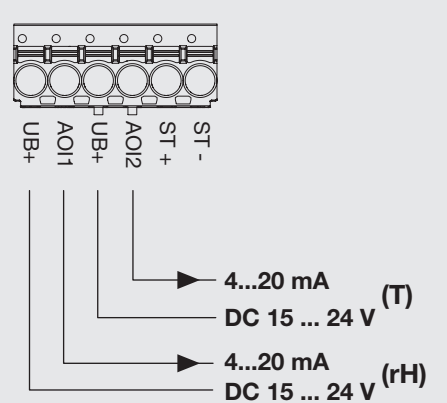
2 x 4...20 mA
