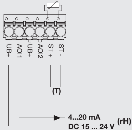
4...20 mA + ST
